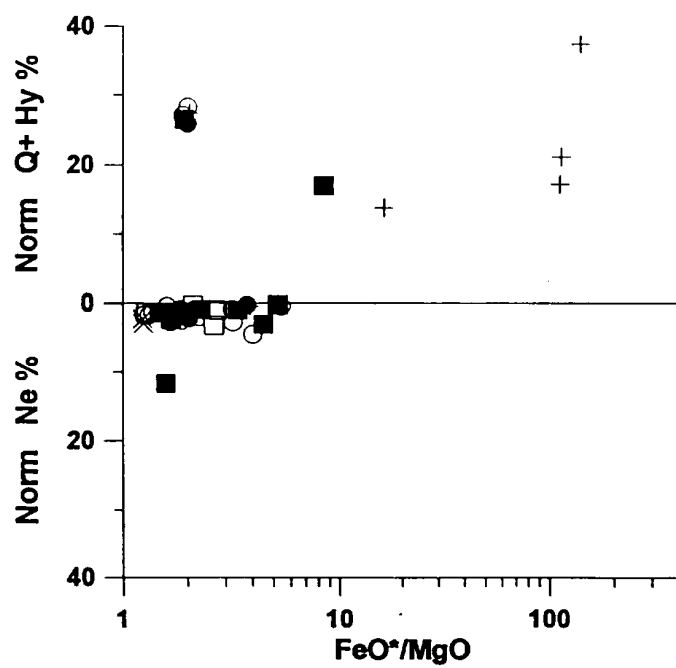
Fig. 68. Plot of \text{FeO}/\text{MgO} vs. norm Q+Hy and Ne. Symbols as in Fig. 62.
